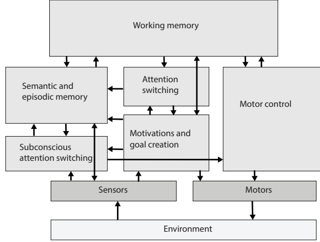
Fig. 1. The general structure of the considered cognitive system
