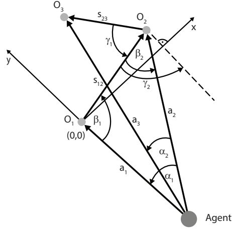
Fig. 4. Adding the third object to the scene map
