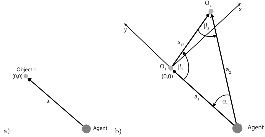
Fig. 3. The first stage of building the scene map: (a) perception of the first object - origin of the local coordinate system, (b) first saccade and location of the second object
